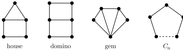
Fig. 2 Forbidden induced subgraphs for distance-hereditary graphs.
